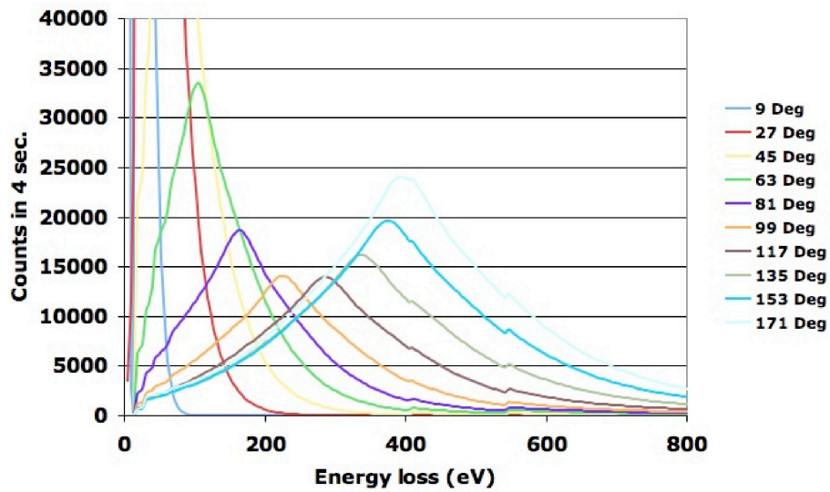
Figure 7. AXIS calculation of the absolute signal level expected in the high-resolution synchrotron measurements of NRIXS of sodium nitrite (Figure 6).
