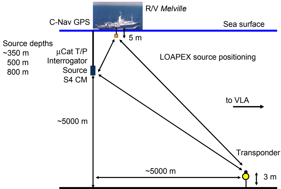
Figure 4.1. LOAPEX source tracking
