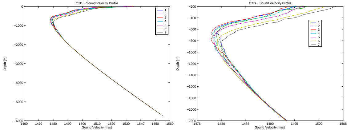
Figure 5.4. Sound speed profiles from the LOAPEX CTD section. Curves 1–7 correspond to stations T50, T250, T500, T1000, T1600, T2300, and T3200. Right panel displays upper ocean variability.
