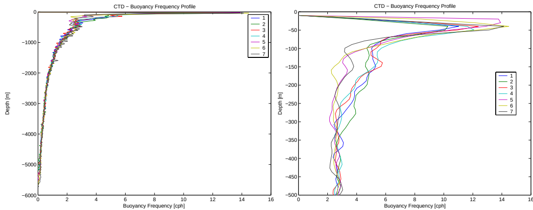
Figure 5.5. Buoyancy frequency profiles from the LOAPEX CTD section. Curves 1–7 correspond to stations T50, T250, T500, T1000, T1600, T2300, and T3200. Right panel displays upper ocean variability.
