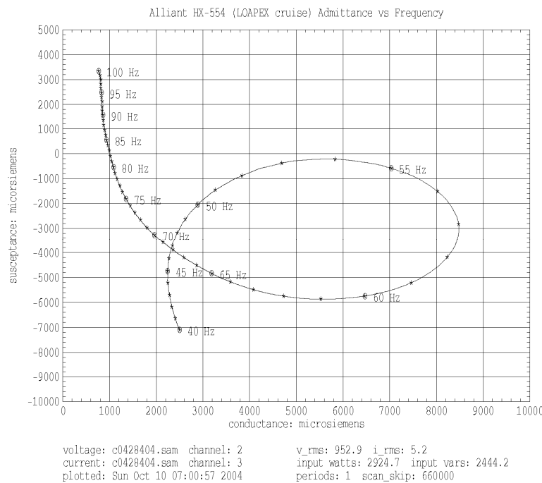
Figure 3.10. Loop plot for 350 m
