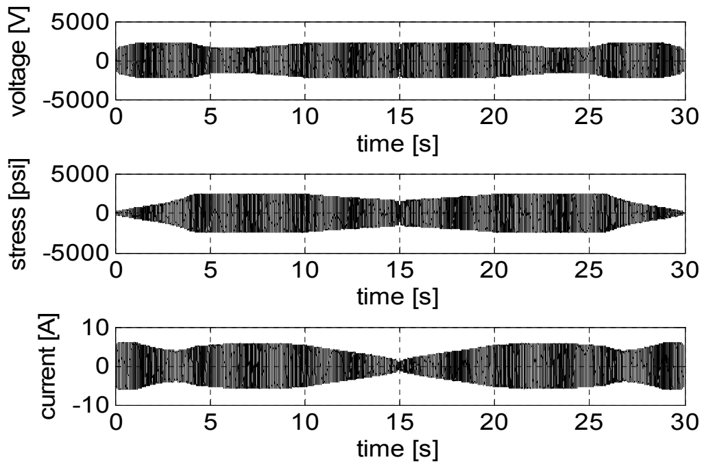
Figure 3.5. Simulated internal waveforms: stack voltage (top), stack stress (middle), tuner current (bottom). These simulations used the input file F195C.800 and the 800Special model.
