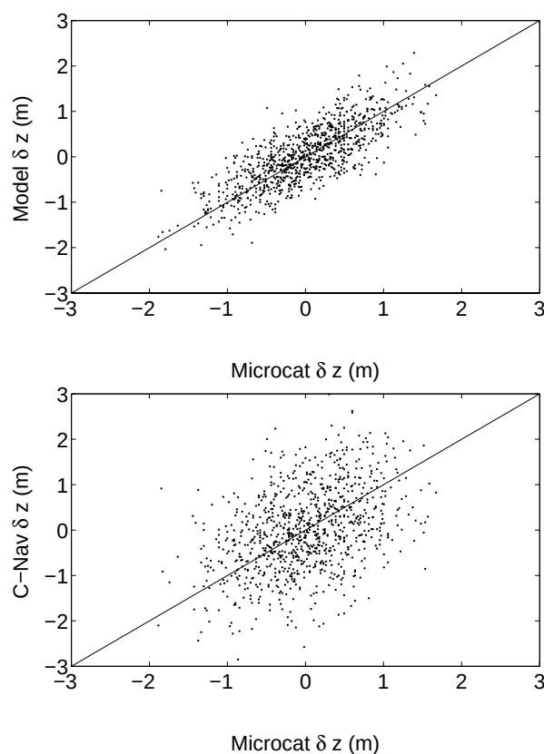
Figure 4.7. Modeled (using C-Nav) vs. measured (MicroCat) vertical source motion (top) and C-Nav vs. MicroCat vertical motion (bottom)
