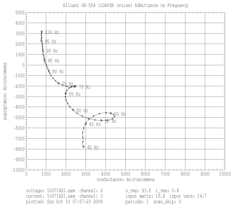
Figure 3.12. Loop plot taken at 800 m during pressurization; interior cavity partially filled
