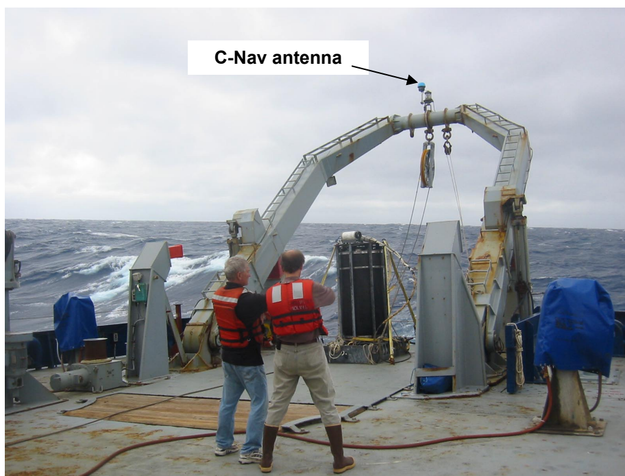
Figure 4.2. The blue C-Nav antenna is next to the navigation light at the center of the A-frame.
