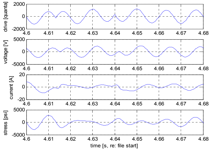
Figure 3.1. A plot of a short segment of M195.800 (top) followed by simulated responses in the stack voltage (second from top), auto-tuner current (third from top), and stack stress (bottom)
