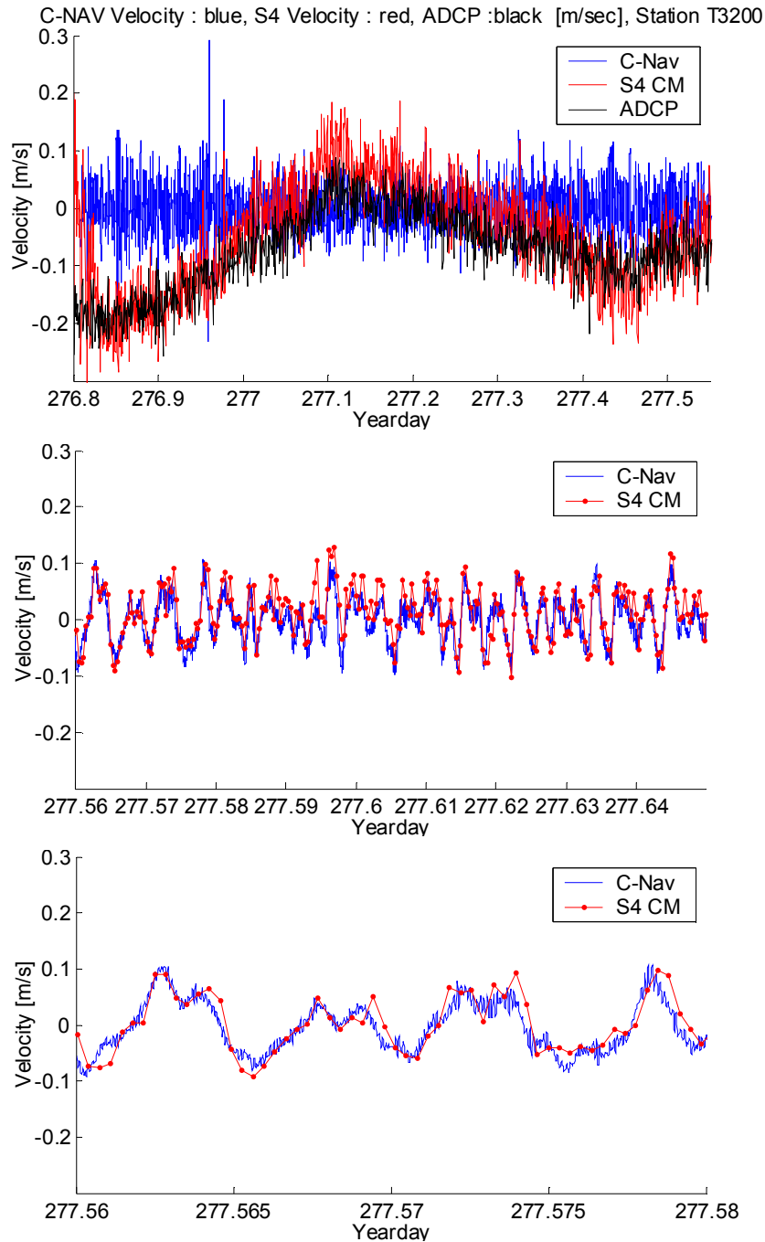
Figure 4.10. S-4 current meter, ADCP, and C-Nav velocities
