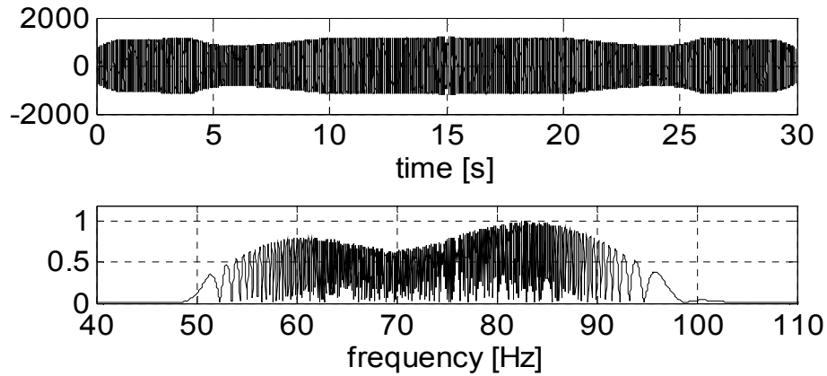
Figure 3.4. Time domain waveform (top) and magnitude Fourier transform (bottom), file F195C.800. The oscillations are too dense in the top panel to be seen individually.
