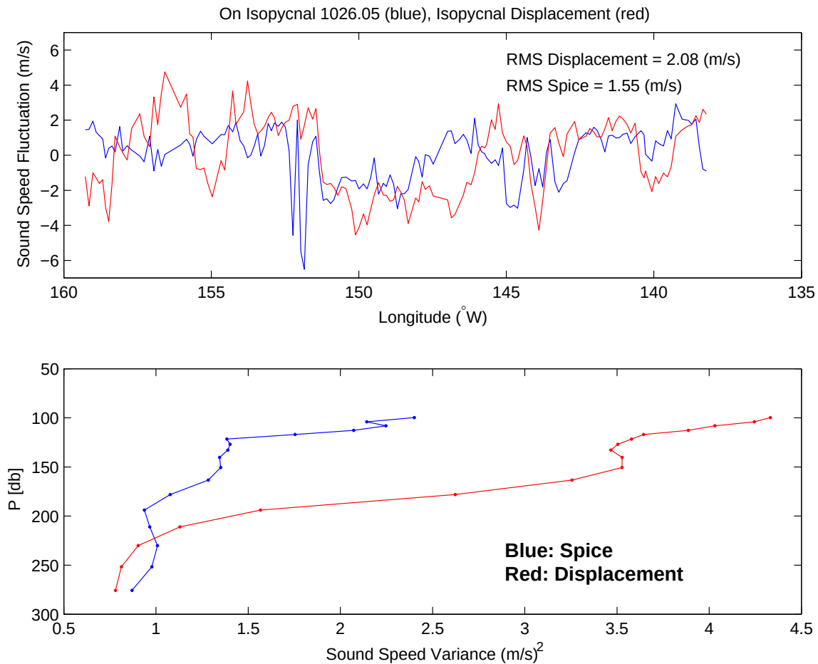
Figure 5.3. Separation of intrusive and displacement effects on sound speed. Upper panel shows an example of sound speed fluctuation along the 1026.05-kg m -3 isopycnal, and the corresponding sound speed fluctuation of that isopycnal displacement relative to the mean sound speed profile. Lower panel shows sound speed variance separated into intrusive and displacement contributions as a function of depth (mean isopycnal displacement).
